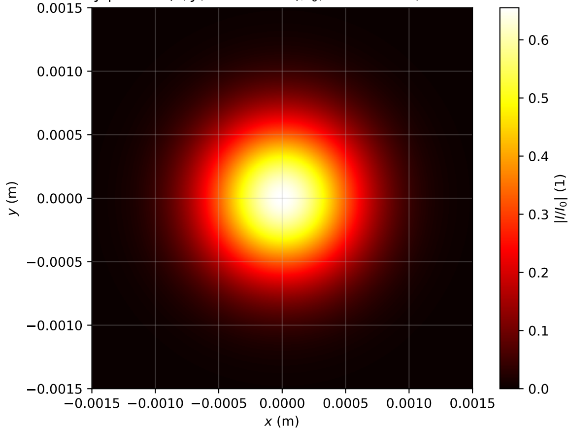
Intensity profile I(x, y, z = 1.592m)/I_0 , Pin=0.1Pcr, artificial time
